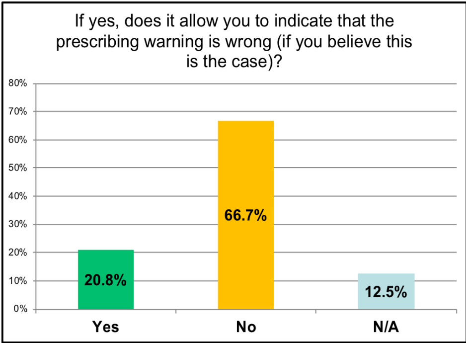
Supplementary Figure 9
