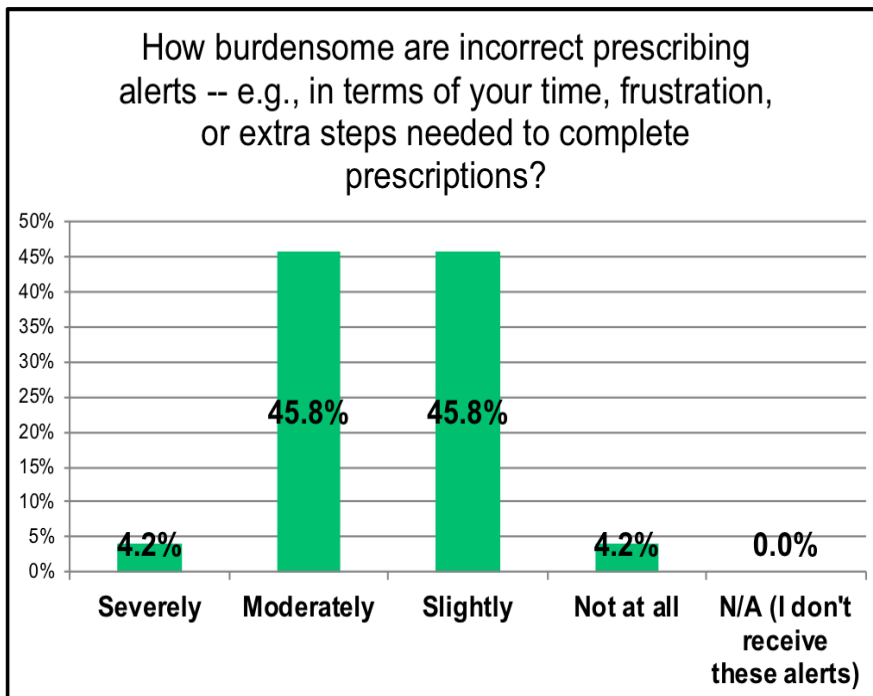
Supplementary Figure 6
