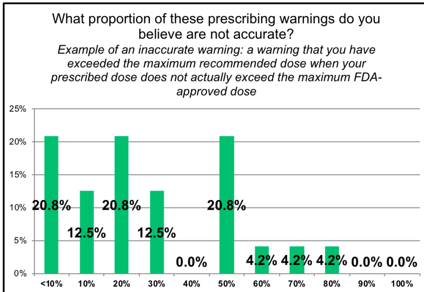
Supplementary Figure 5
