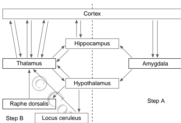
Figure 2. Scheme of the Functional Organization of the Brain*
