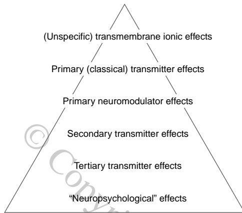
Figure 1. Hierarchy of Mood-Stabilizing Mechanisms*
