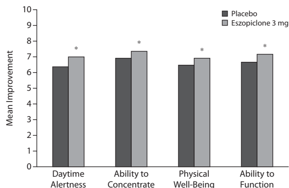
Figure 2. Daytime Functioning: Mean Double-Blind Averages a
