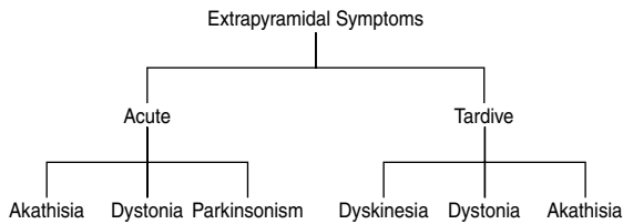
Figure 1. Neuroleptic-Induced EPS*
