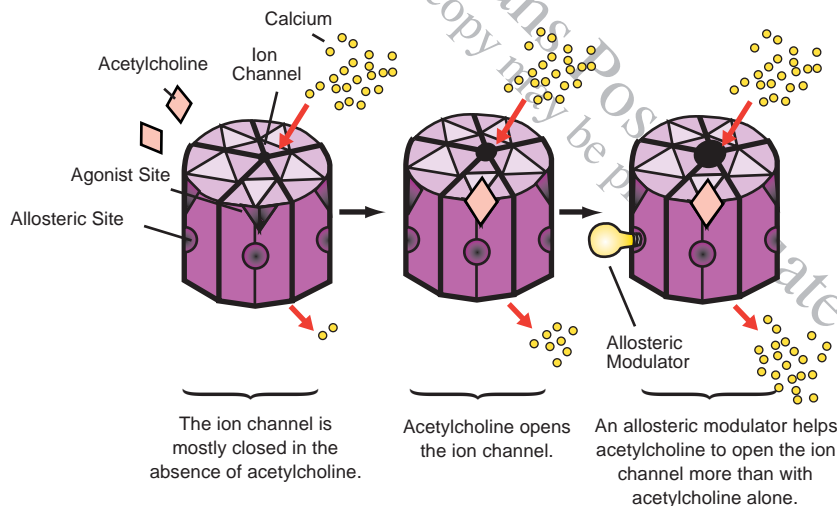
Figure 2. Opening an Ion Channel With Acetylcholine
