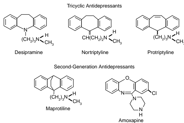
Figure 2. Structures of Drugs That Selectively Block the Reuptake of Norepinephrine a
