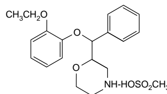
Figure 3. The Structure of Reboxetine, (2RS, \alpha RS)-2-[ \alpha -2-(ethoxyphenoxy)benzyl] Morpholine Methanesulphonate a
