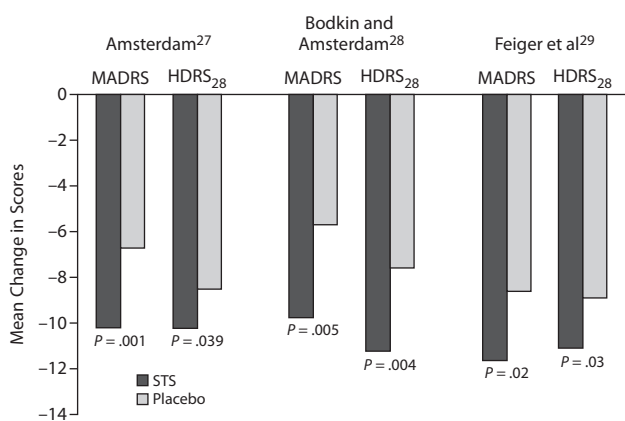
Figure 1. Mean Change From Baseline in MADRS and HDRS 28 Scores for Patients Treated With Transdermal Selegiline Versus Placebo
